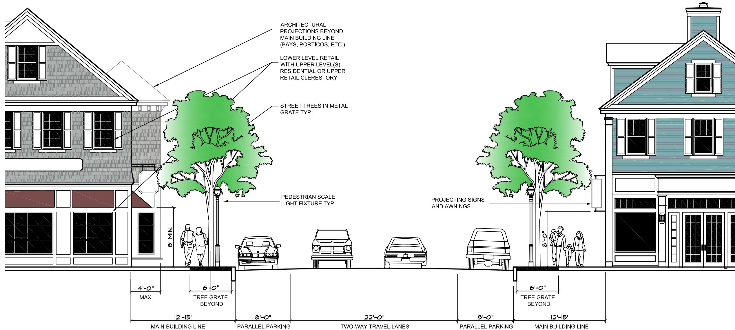
TYPICAL SIDE STREET SECTION WITH PARALLEL PARKING
