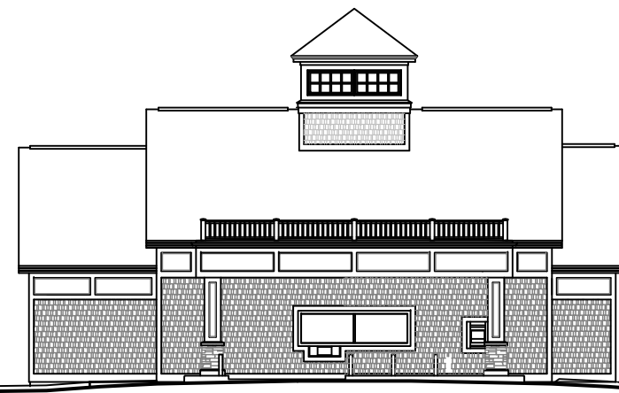
NORTH ELEVATION
